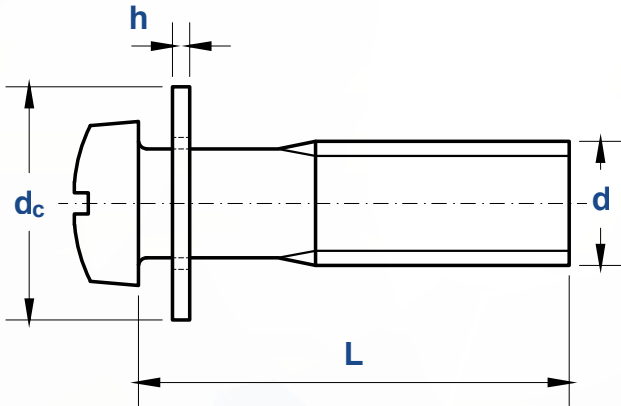
Screw with shank
