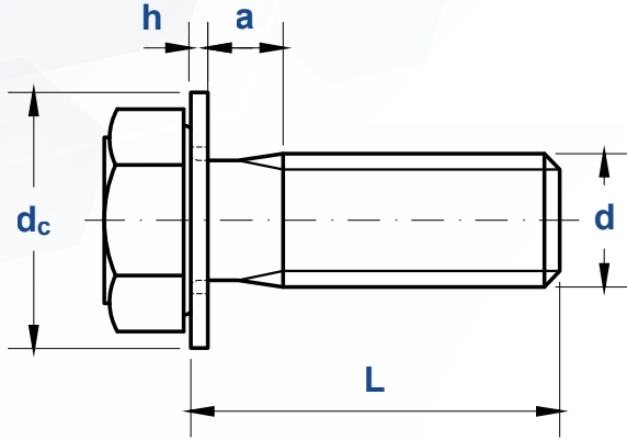
Screw threaded up to the washer
