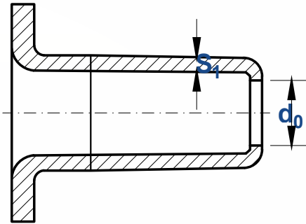
(C2) Made from strip
