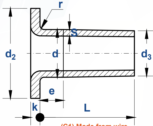
(C1) Made from wire
