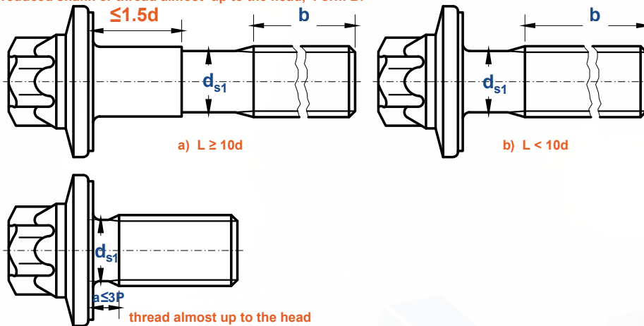
Screw with reduced shank or thread almost up to the head, Form B:
